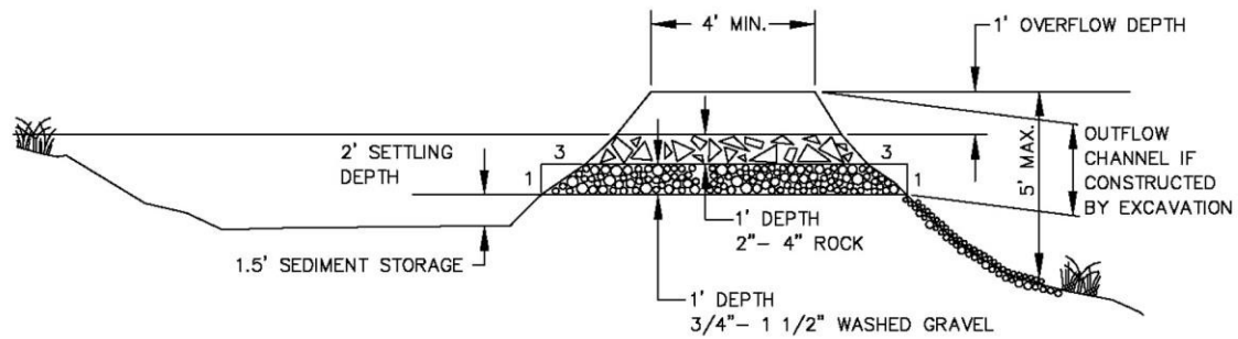
CROSS SECTION
